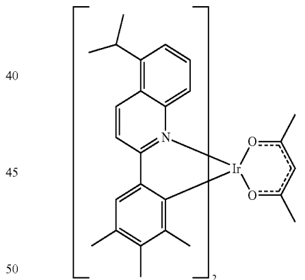
Compound 42
