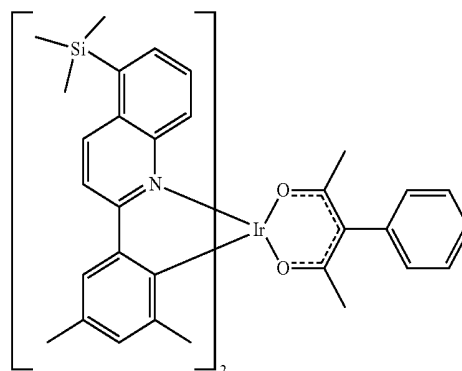
Compound 14
