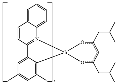
Compound C
