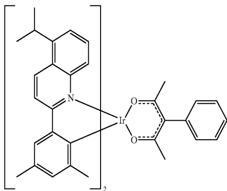
Compound 21
